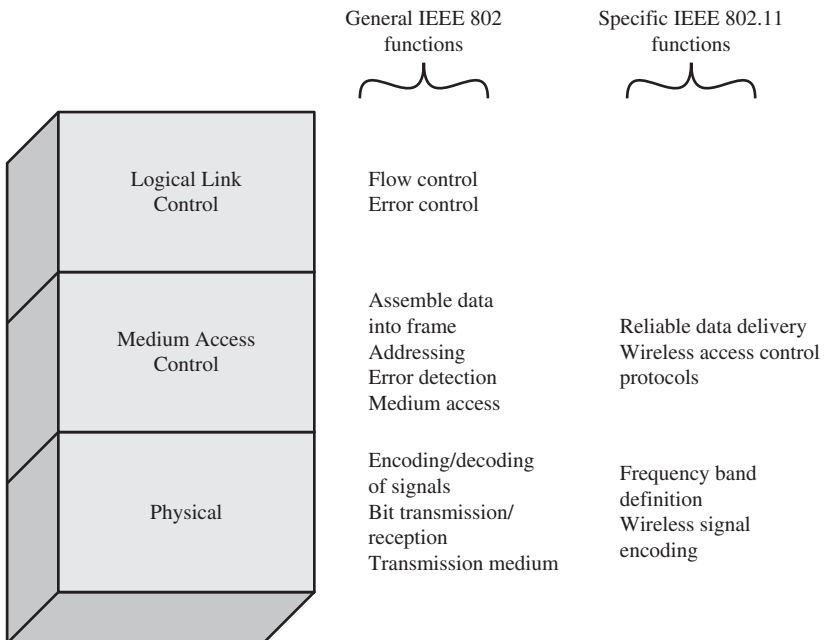
Figure 24.2 IEEE 802.11 Protocol Stack
