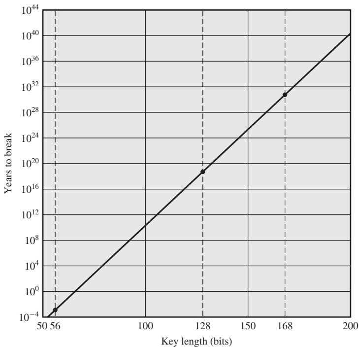
Figure 2.2 Time to Break a Code (assuming 10^6 decryptions/ \mu\text{s} ) The graph assumes that a symmetric encryption algorithm is attacked using a brute-force approach of trying all possible keys
