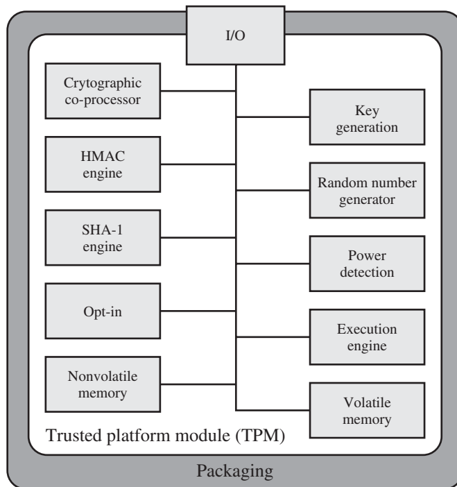
Figure 13.12 TPM Component Architecture
