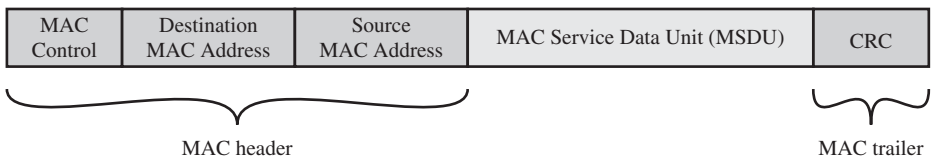
Figure 24.3 General IEEE 802 MPDU Format
