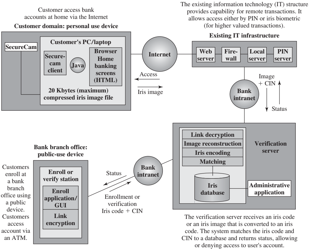
Figure 3.11 Multichannel System Architecture Used to Link Public- and Personal-Use Iris Identification Devices via the Internet The system uses each customer's PIN (personal identification number), iris code, and CIN (customer identification number) to validate transactions. Source: [NEGI00]
