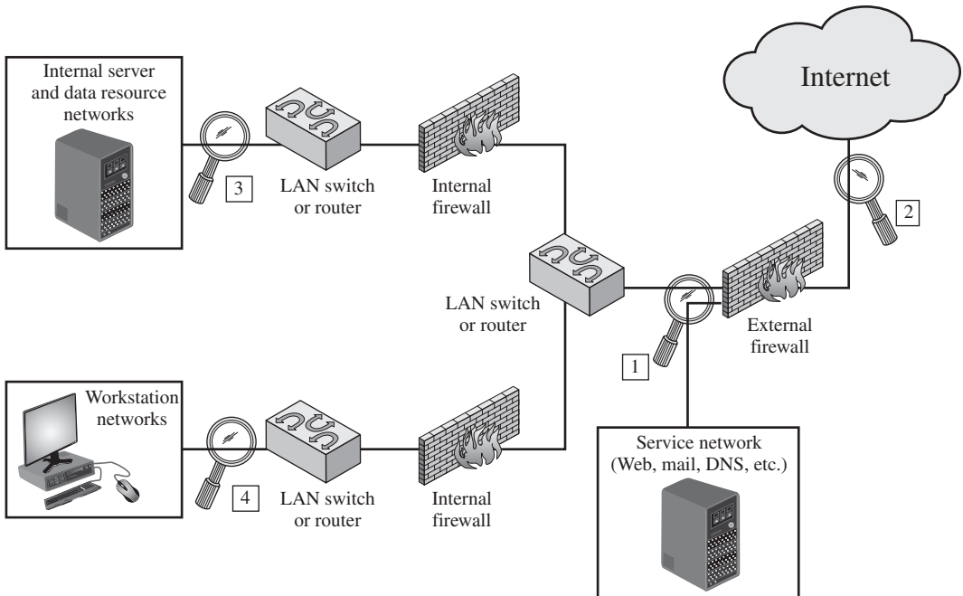
Figure 8.5 Example of NIDS Sensor Deployment
