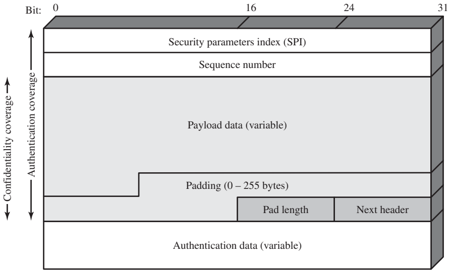
Figure 22.7 IPsec ESP Format
