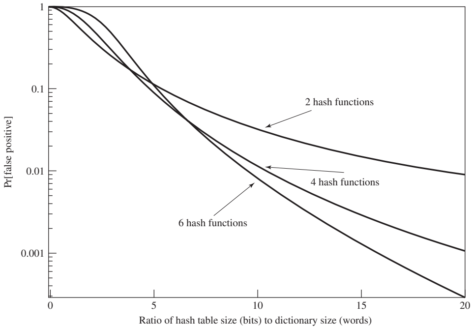
Figure 3.2 Performance of Bloom Filter
