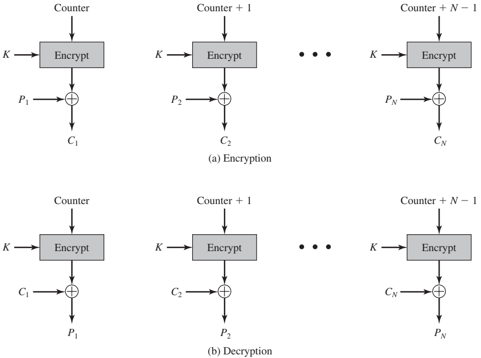
Figure 20.8 Counter (CTR) Mode
