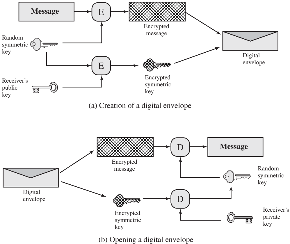
Figure 2.9 Digital Envelopes
