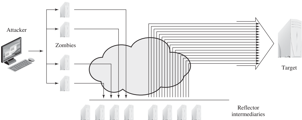
Figure 7.7 Amplification Attack
