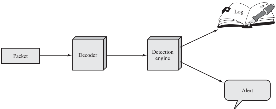
Figure 8.9 Snort Architecture
