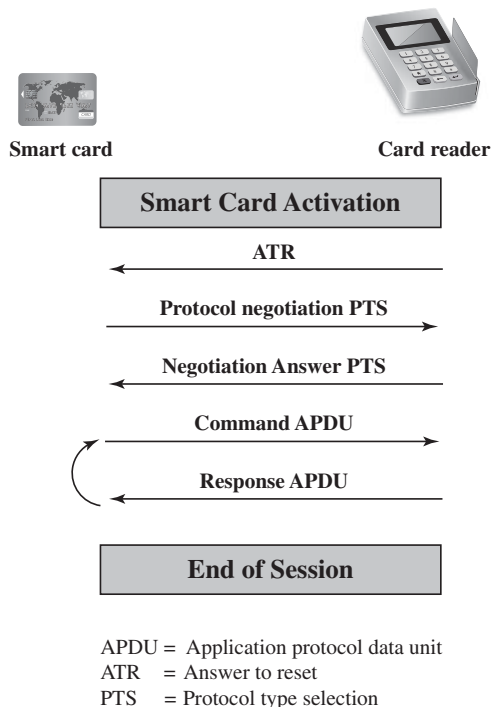
Figure 3.4 Smart Card/Reader Exchange
