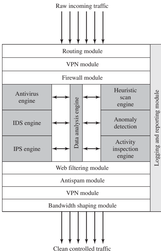
Figure 9.5 Unified Threat Management Appliance
