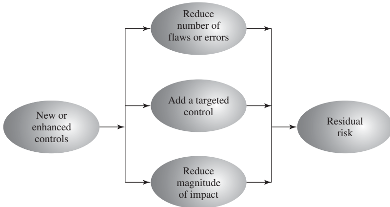
Figure 15.3 Residual Risk
