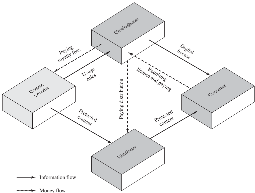
Figure 19.3 DRM Components
