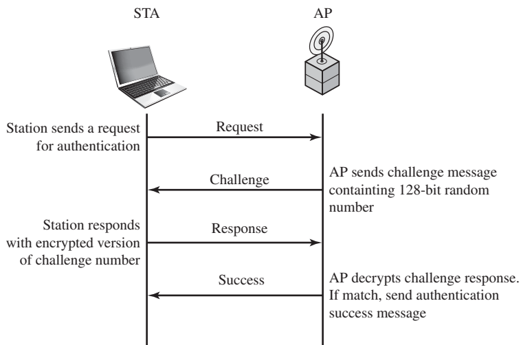
Figure 24.12 WEP Authentication
