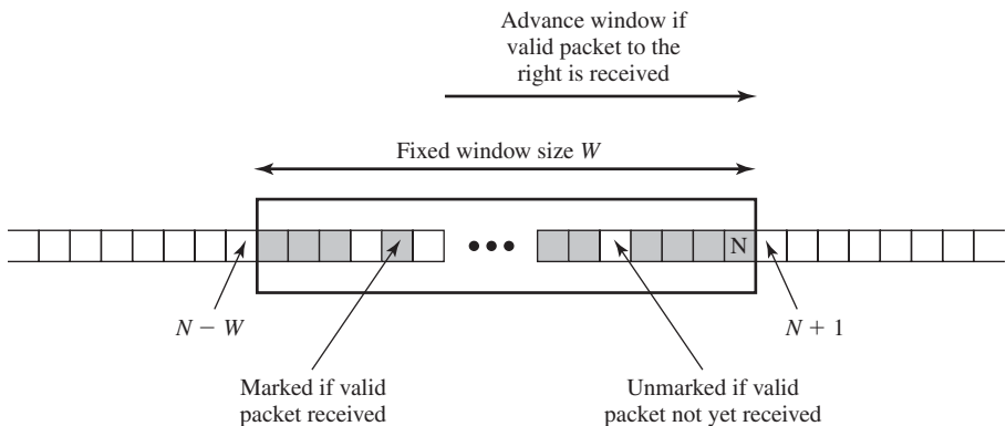
Figure 22.8 Antireplay Mechanism
