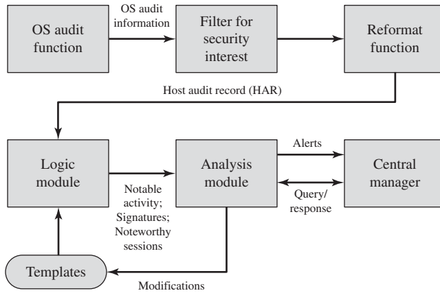
Figure 8.3 Agent Architecture
