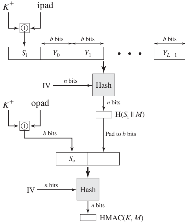
Figure 21.4 HMAC Structure
