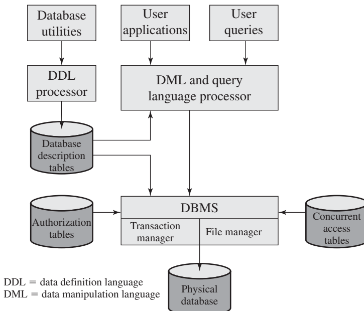
Figure 5.1 DBMS Architecture
