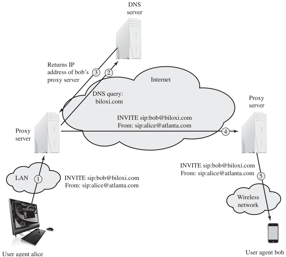
Figure 7.5 SIP INVITE Scenario
