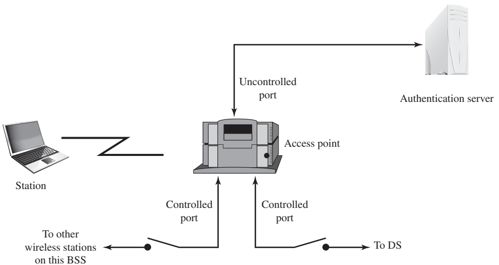
Figure 24.8 802.1X Access Control
