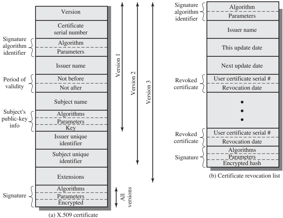
Figure 23.3 X.509 Formats
