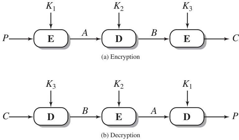
Figure 20.2 Triple DES
